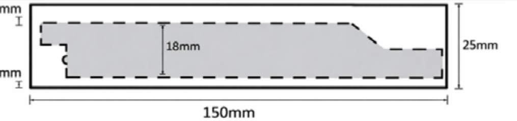
18 mm thick cladding produced from 25mm Accoya
