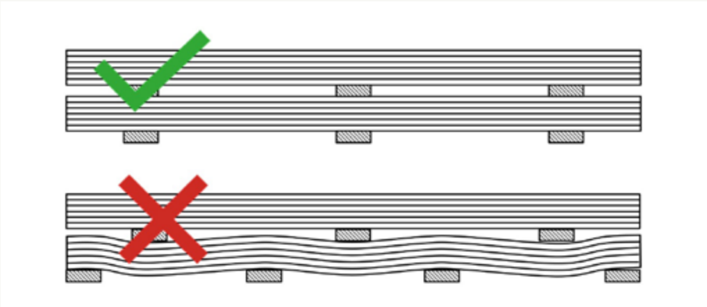
Bundles stored on top of each other; bearers aligned
